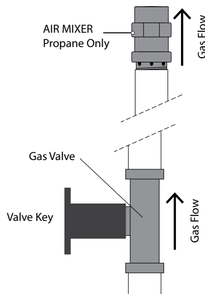
FIGURE 2: VALVE CONNECTIONS
